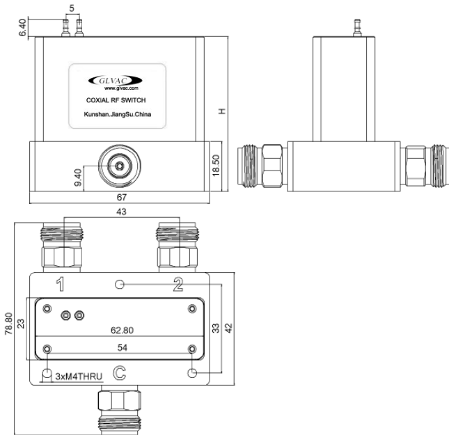
H=58mm(max)
